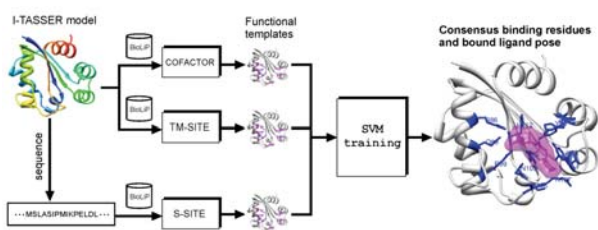
Figure D. Flowchart of COACH for ligand binding site prediction. The final results are combined from the complementary predictions by COFACTOR, TM-SITE and S-SITE using support vector machine (SVM).
