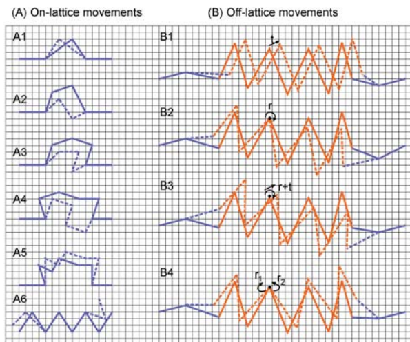
Figure B. Conformational movements in the I-TASSER Monte Carlo simulations. Solid and dashed lines are C \alpha traces before and after movements. Blue lines represent the threading unaligned regions with moves on the lattice system and orange ones are from the aligned regions with moves off-lattice. Left Panel: (A1) two bond vector random walk; (A2) three bond vector walk; (A3) four bond vector walk; (A4) five bond vector walk; (A5) six bond vector translation; (A6) N- and C-terminal random walk. Right Panel: (B1) fragment translation; (B2) fragment rotation around a random residue; (B3) fragment rotation and translation; (B4) small deformation of a fragment. After each fragment movement, the neighboring vectors at the two ends are regenerated to keep the chain connection.
