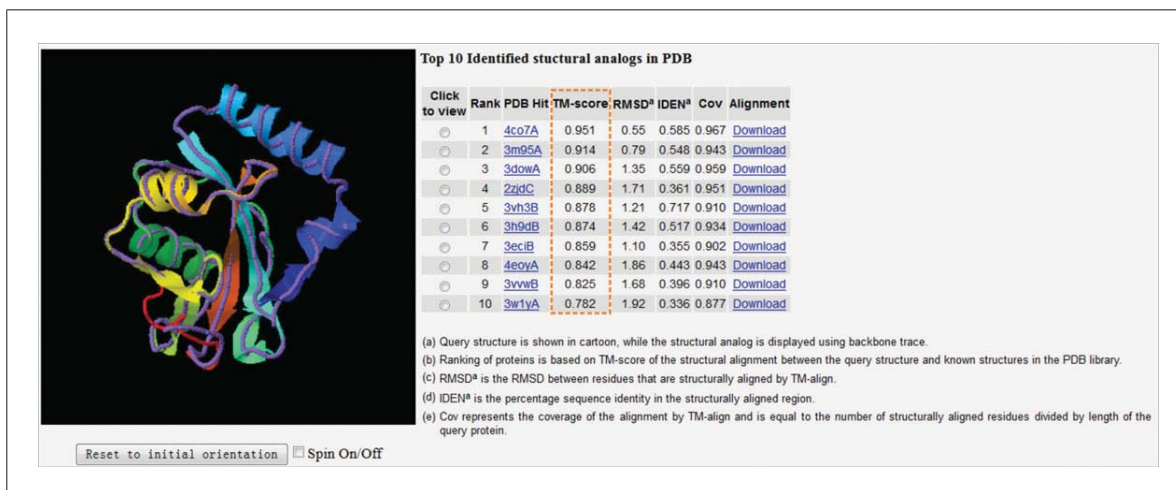
Figure 5.8.7 Ten PDB structures close to the target. The structure of the first I-TASSER model (model 1, shown in rainbow cartoon) is superimposed on the analogous structures from the PDB (shown in medium-purple backbone trace). The structural similarity between the target model and the 10 closest proteins are ranked by TM-scores, which are highlighted in the orange box. The coordinate file of the superimposed structures can be downloaded through the Download link for local visualization. In this example, there are multiple analogous structures from the PDB that have a high TM-score (>0.9), including 4co7A, 3m95A, and 3dowA. However, it is also possible that no similar structures can be found in the PDB; this usually indicates that the target protein is a new-fold protein or the fold by I-TASSER prediction is not correct.
