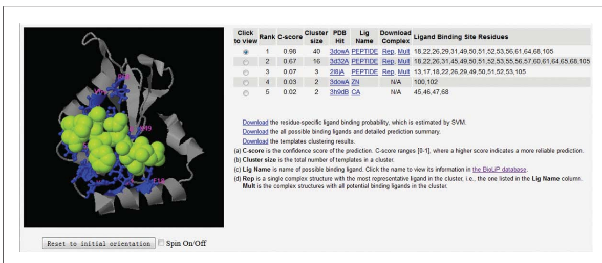
Figure 5.8.8 Illustration of ligand binding site prediction. The binding site prediction shown on the table is made by COACH, which combines the prediction results from five complementary algorithms of COFACTOR (Roy et al., 2012), TM-SITE, S-SITE (Yang et al., 2013b), FindSite (Brylinski and Skolnick, 2008), and ConCavity (Capra et al., 2009). The predicted binding ligand is highlighted in yellow-green spheres, with the corresponding binding residues shown as blue ball-and-stick illustrations in the picture of the 3-D model. In this example, the first functional template (PDB ID: 3dowA) has a high confidence score (C-score = 0.98) that it binds with a peptide ligand. Except for the predicted peptide, the protein can also bind to other ligands, which are available in a PDB file at the 'Mult' link. The ligands separated by 'TER' are put in the end of this file.
