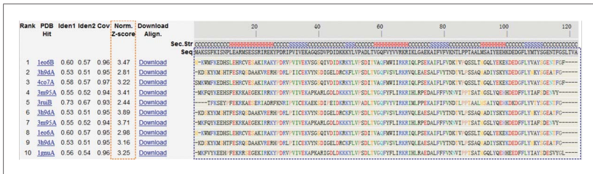
Figure 5.8.5 The top 10 threading templates used by I-TASSER. The Z-score, which has been widely used for estimating the significance and the quality of template alignments, equals the difference between the raw alignment score and the mean in units of standard deviation. However, since LOMETS contains templates from multiple threading programs where the Z-scores are not comparable between different programs, I-TASSER uses a normalized Z-score (highlighted by the orange box) to specify the quality of the template, which is defined as the Z-score divided by the program-specific Z-score cutoffs. Thus, a normalized Z-score >1 indicates an alignment with high confidence. In this example, because there are multiple templates with the normalized Z-score above 1, the target is categorized by I-TASSER as an ‘Easy’ target. The multiple alignments between the query and the templates are marked by the blue box, where the residue numbers of each template are available by clicking on the corresponding ‘Download’ link. It can be seen from the multiple sequence alignment that, except for a few residues at the N- and C- terminals of the query (i.e., aligned to gaps ‘-’), other residues are well aligned with templates. This usually indicates that there is a high level of conservation between the target and templates.
